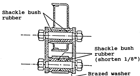
Figure 5 – Front spring, rear shackle
